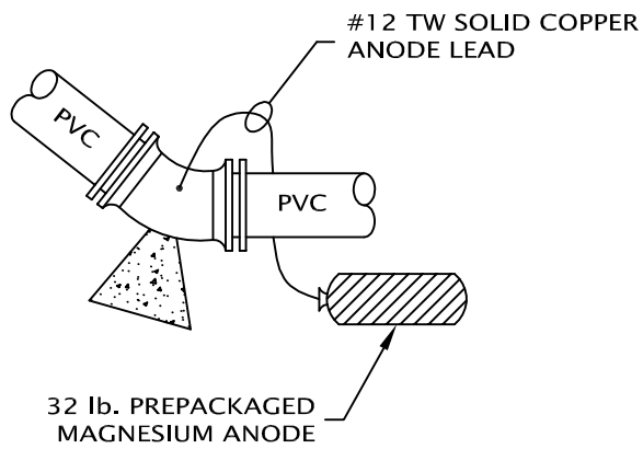
TYPICAL PIPE BEND
