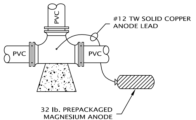
TYPICAL PIPE TEE
